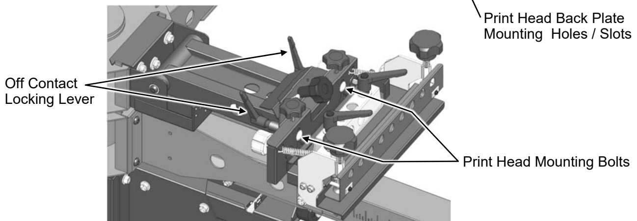
Print Head Installed
