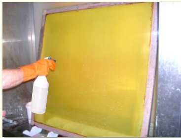
1) After removal of ink, block-out, and emulsion, apply ENVIROCLEAN® to the screen (both sides).
